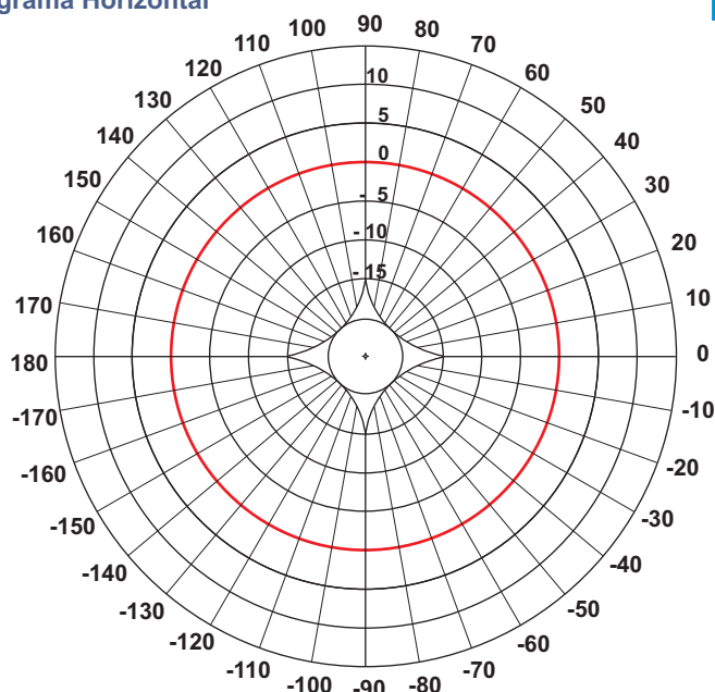
Diagrama Horizontal
