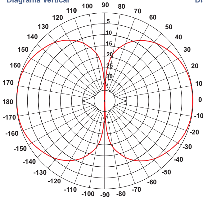
Diagrama Vertical
