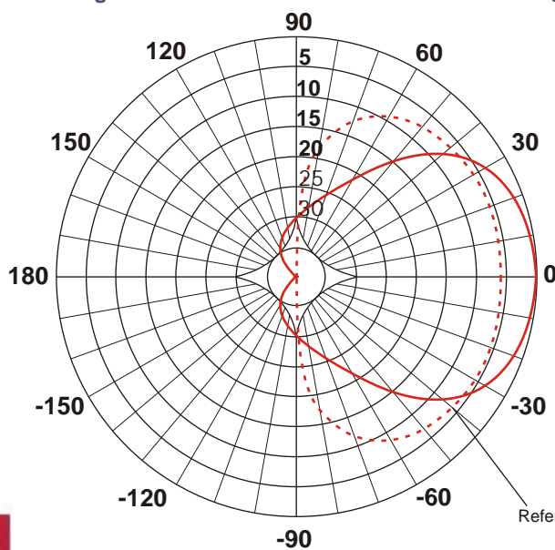
Diagrama Vertical
