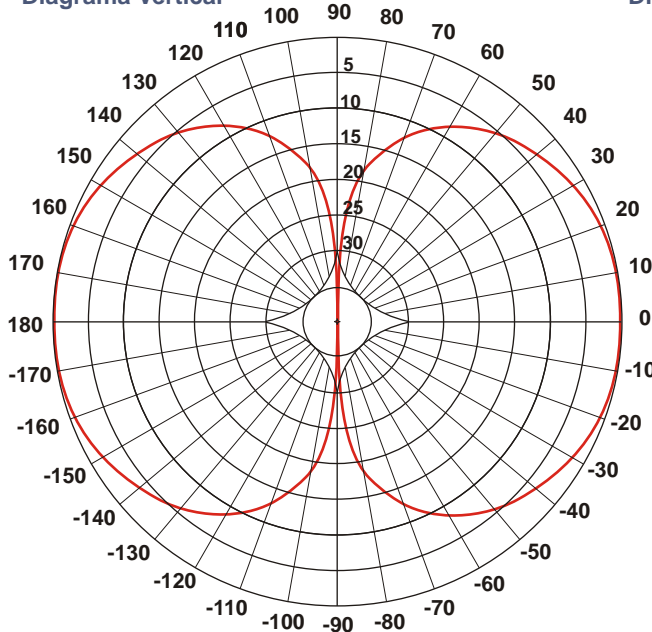
Diagrama Vertical
