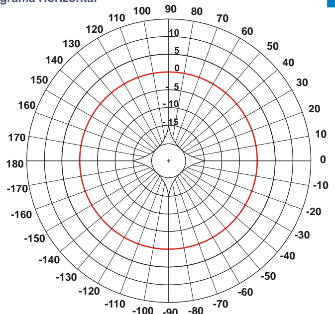
Diagrama Horizontal
