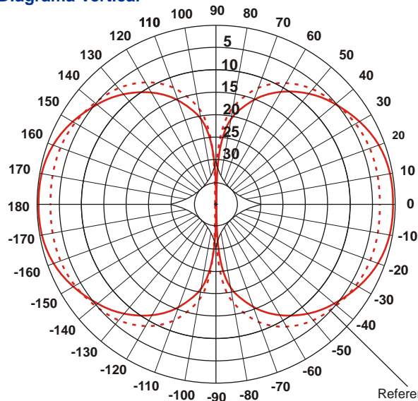
Diagrama Vertical
