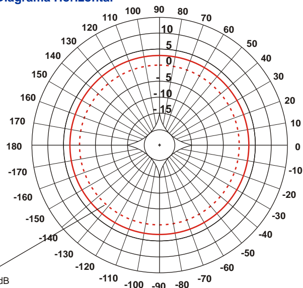
Diagrama Horizontal
